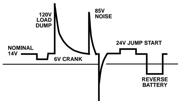
FIGURE 1. TYPICAL AUTOMOTIVE TRANSIENTS
