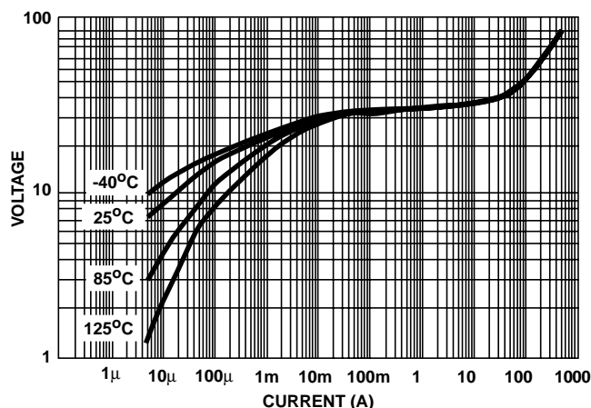
FIGURE 9. TYPICAL V - I CHARACTERISTICS OF THE V18AUMLA2220 AT -40^\circ\text{C} , 25^\circ\text{C} , 85^\circ\text{C} AND 125^\circ\text{C}
