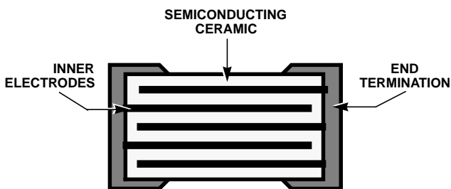
FIGURE 4. AUML INNER CONSTRUCTION
