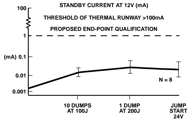
FIGURE 2D. STABILITY OF STANDBY CURRENT
