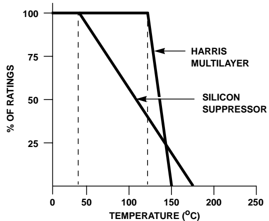
FIGURE 14. AURL AND SILICON SUPPRESSORS CURRENT, ENERGY AND POWER DERATING CURVE
