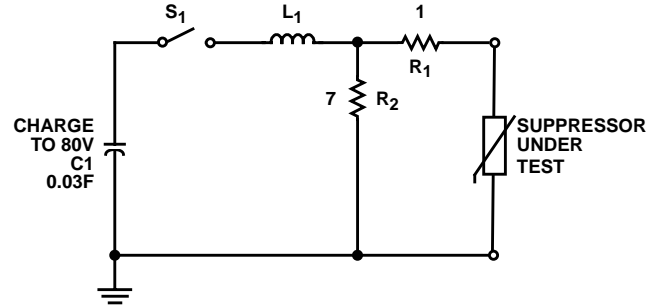
FIGURE 2B. LOAD DUMP SIMULATOR CIRCUIT
