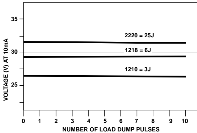
FIGURE 5. LOAD DUMP PULSING OVER A TEMPERATURE RANGE OF - 55°C TO 125°C
