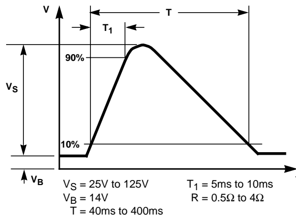
FIGURE 2. LOAD DUMP TRANSIENT
