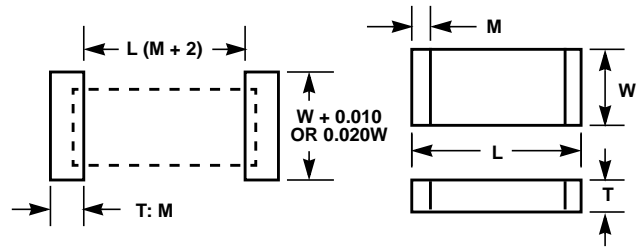
FIGURE 10. LAND PAD PATTERNS FOR MULTILAYER SUPPRESSORS
