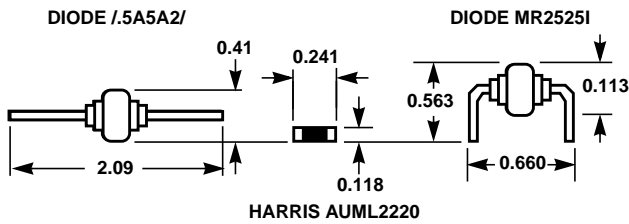
FIGURE 15. SIZE COMPARISONS OF AUTOMOTIVE SURGE SUPPRESSORS
