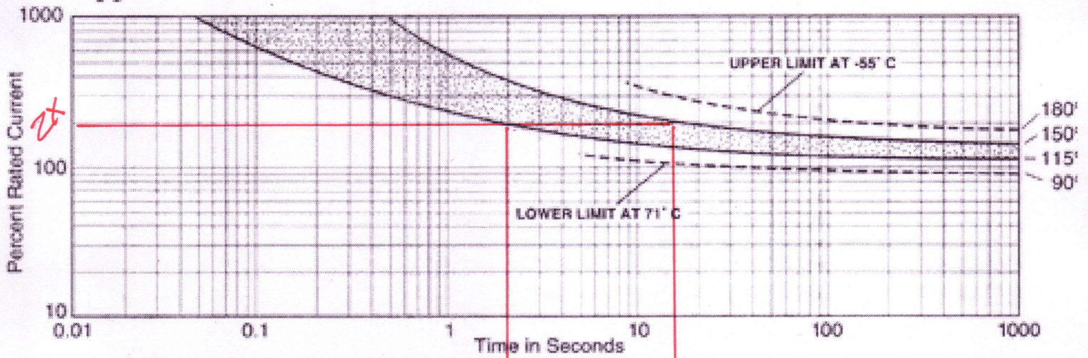
Approximate Time-Current Curves at 25°C
