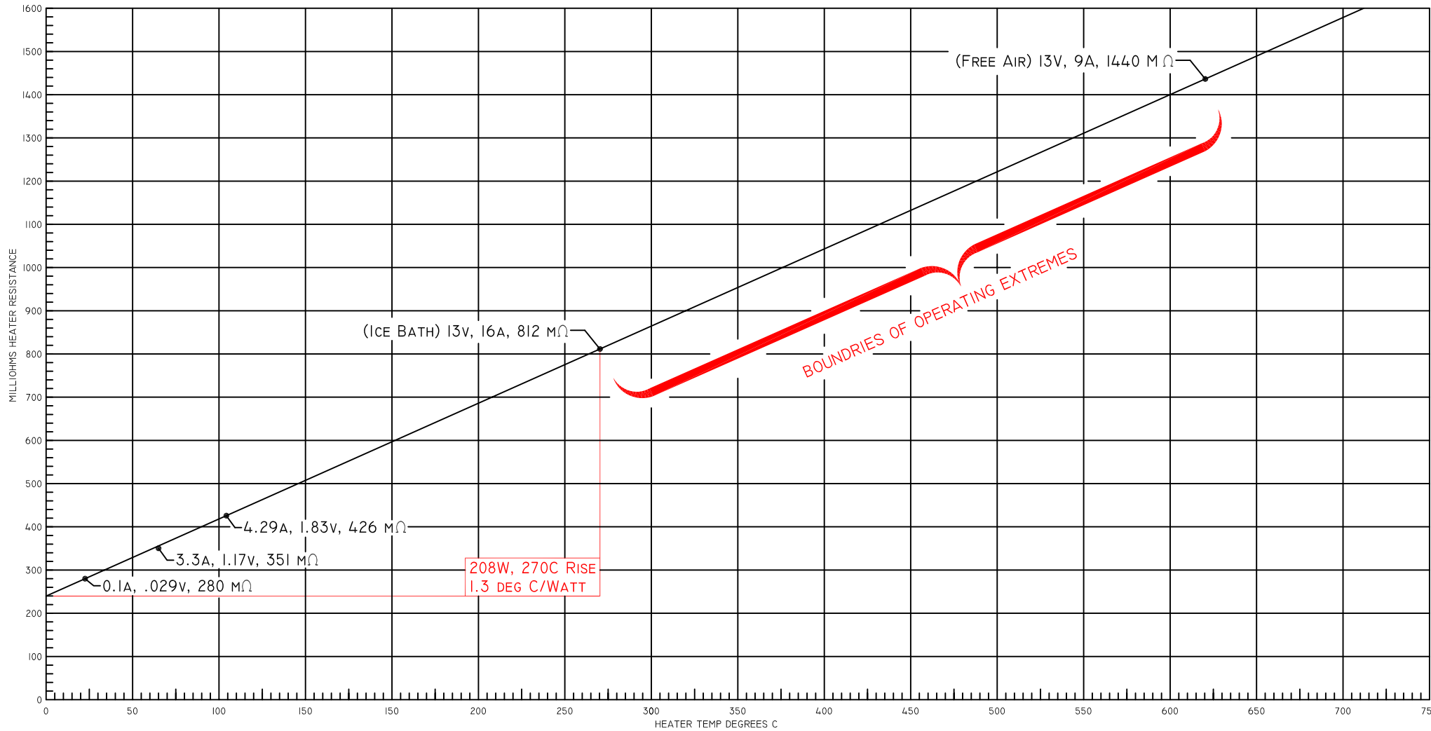
AN5814-I PITOT TUBE R-TEMP CURVE
