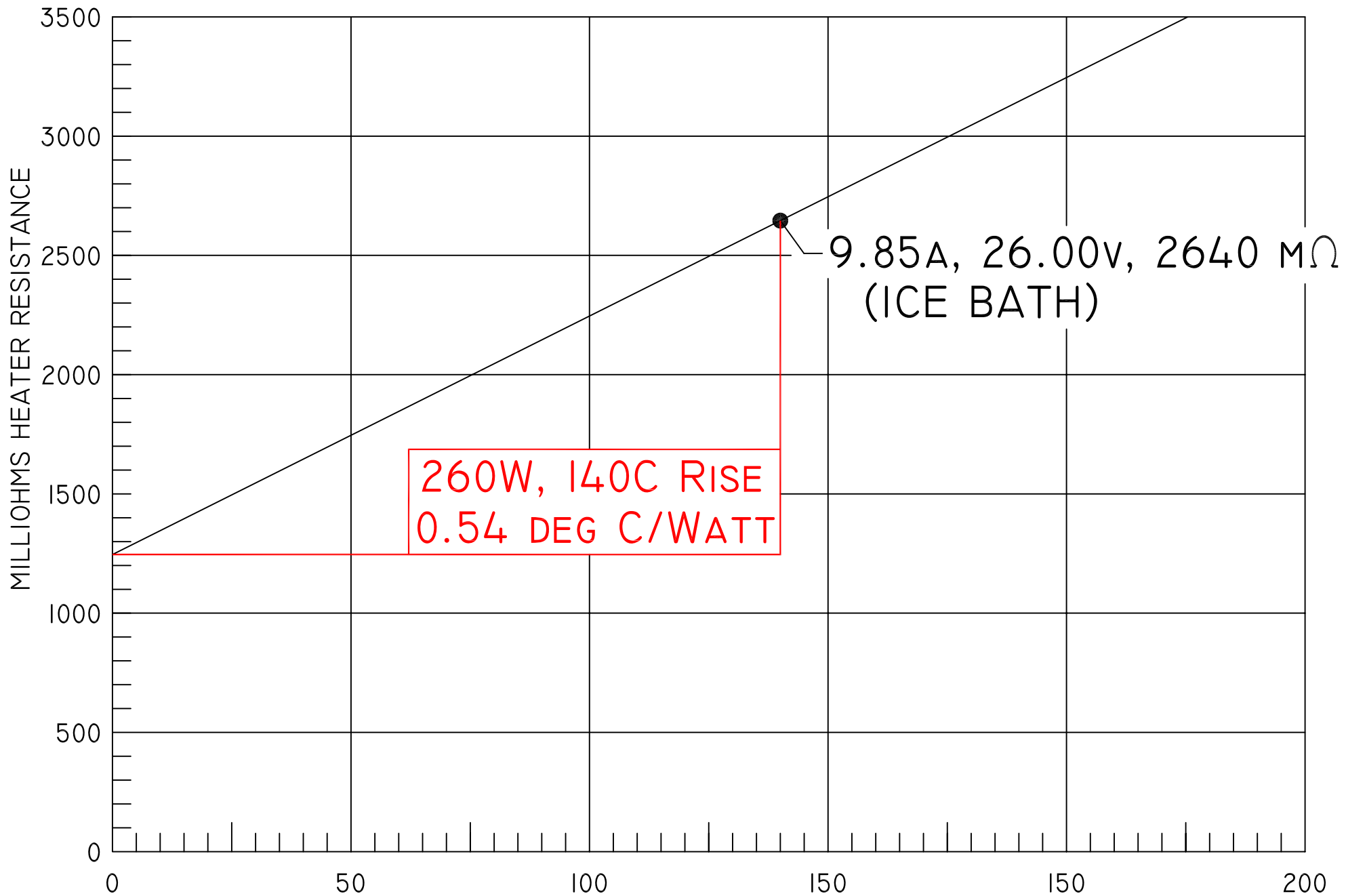
HEATER TEMP DEGREES C 26V PITOT TUBE R-TEMP CURVE
