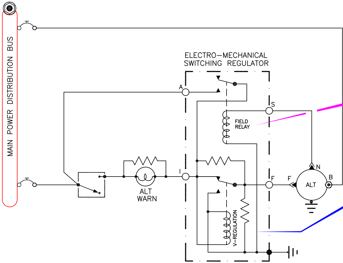
LEGACY ELECTRO-MECHANICAL ALTERNATOR REGULATORS AND FUNCTIONALITY OF THE Y-WOUND STATOR CENTER-TAP
