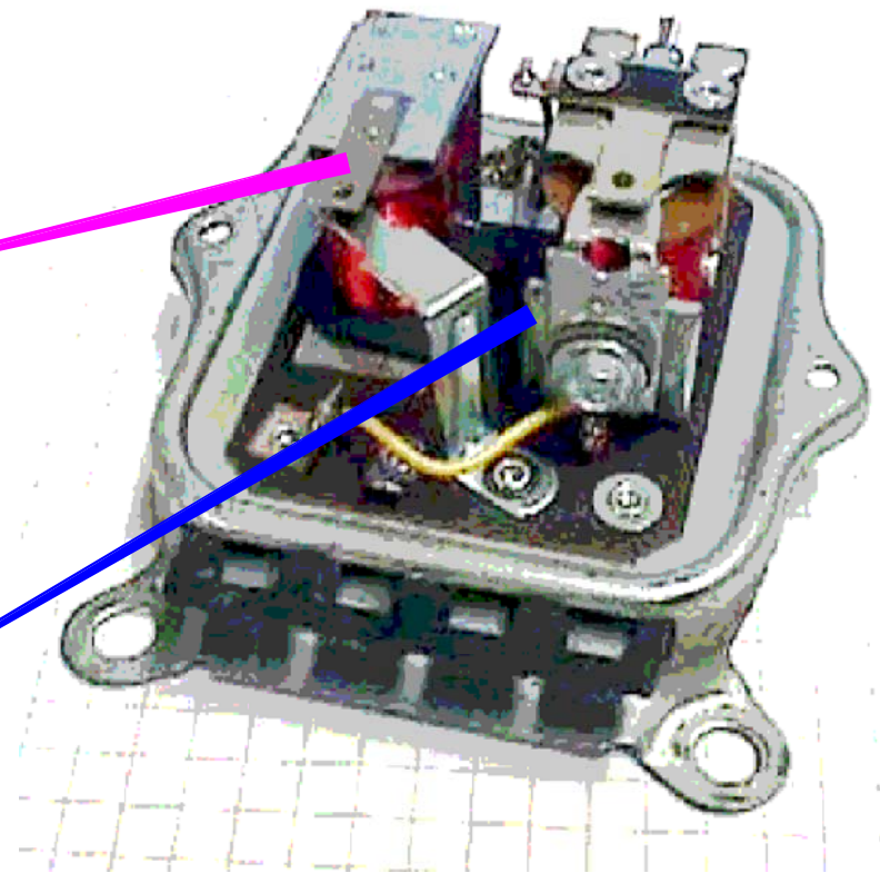
LEGACY ELECTRO-MECHANICAL ALTERNATOR REGULATORS AND FUNCTIONALITY OF THE Y-WOUND STATOR CENTER-TAP
