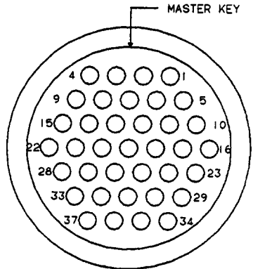
DIAGRAM REF HARNESS SIDE WIRE NO.
