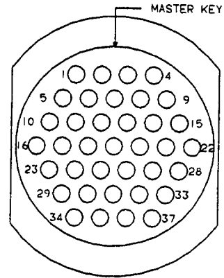
SHIP SIDE WIRE NO. DIAGRAM REF
