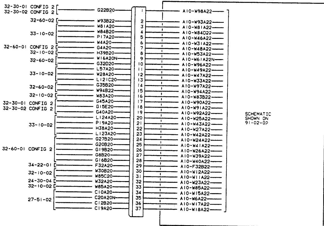
A10 ANNUNCIATOR LIGHT JUNCTION BOX ASSEMBLY
