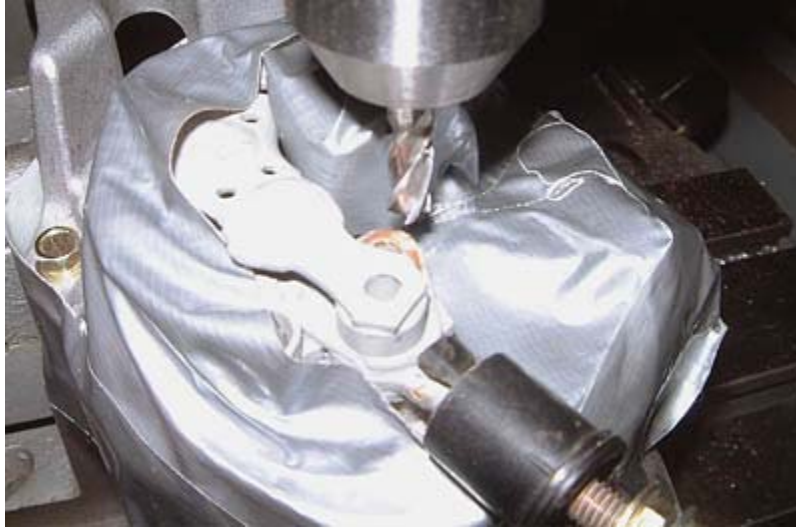
Although this image shows how Lynn used a mill to machine away the copper attachment, a handheld Dremel works fine, too.
